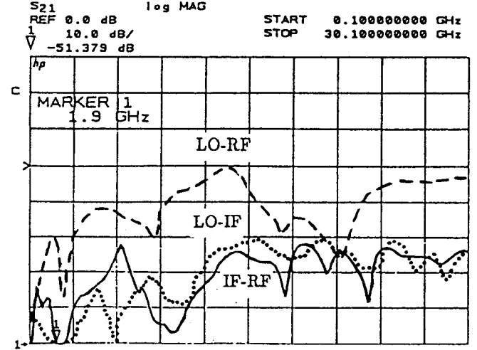
Fig. 3. Upconverter isolation characteristics.
